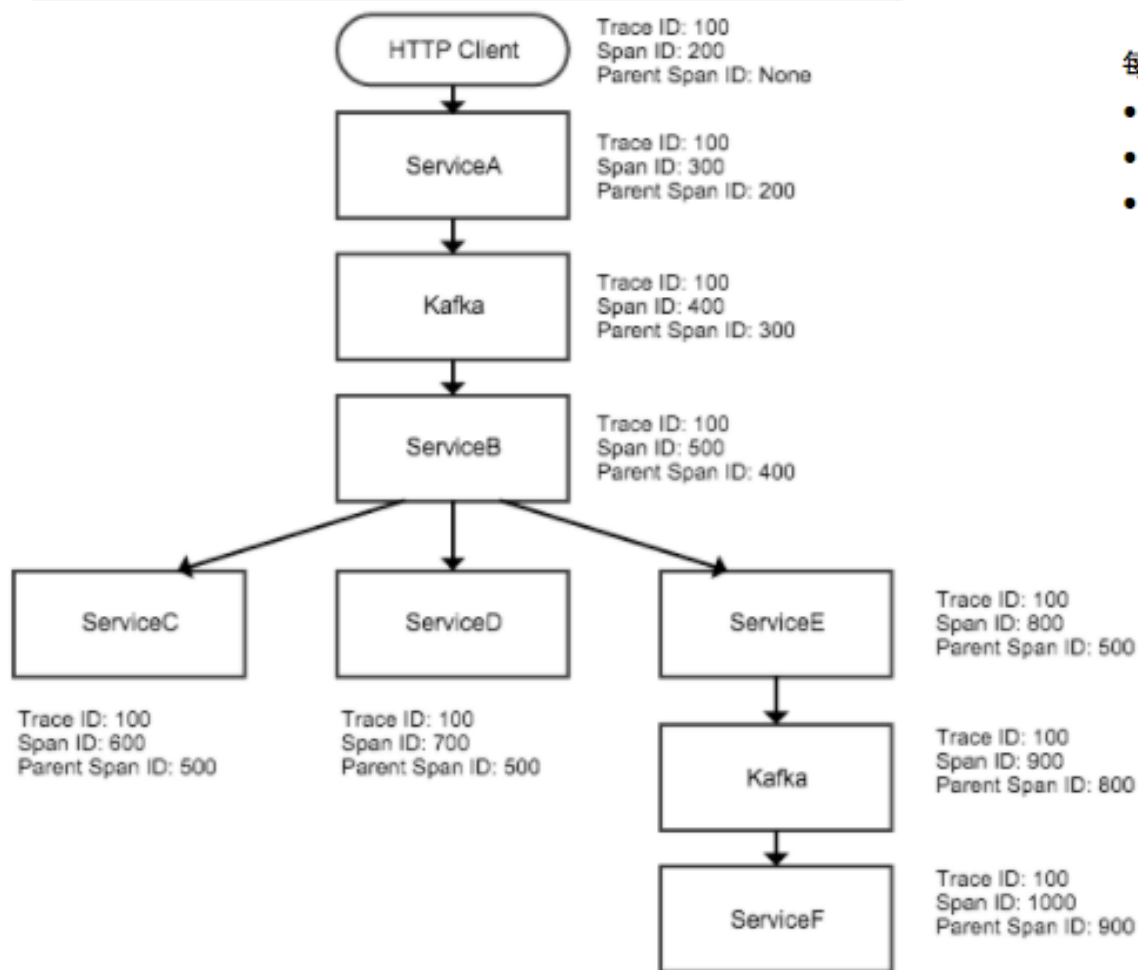
Trace Tree with IDs
